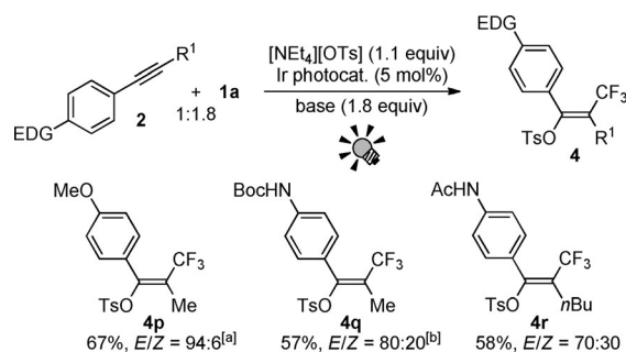
Scheme 2. Photocatalytic trifluoromethyltosylation of alkynes bearing an electron-donating group (EDG). Reaction conditions: [\text{Ir}(\text{ppy})_2\text{-(dtbbpy)}](\text{PF}_6) (5 mol%), 2,6-di- tert -butylpyridine (1.8 equiv). [a] 1a and base (1.5 equiv each) were used. [b] [\text{NMe}_4][\text{OTs}] was used. EDG = electron-donating group.
